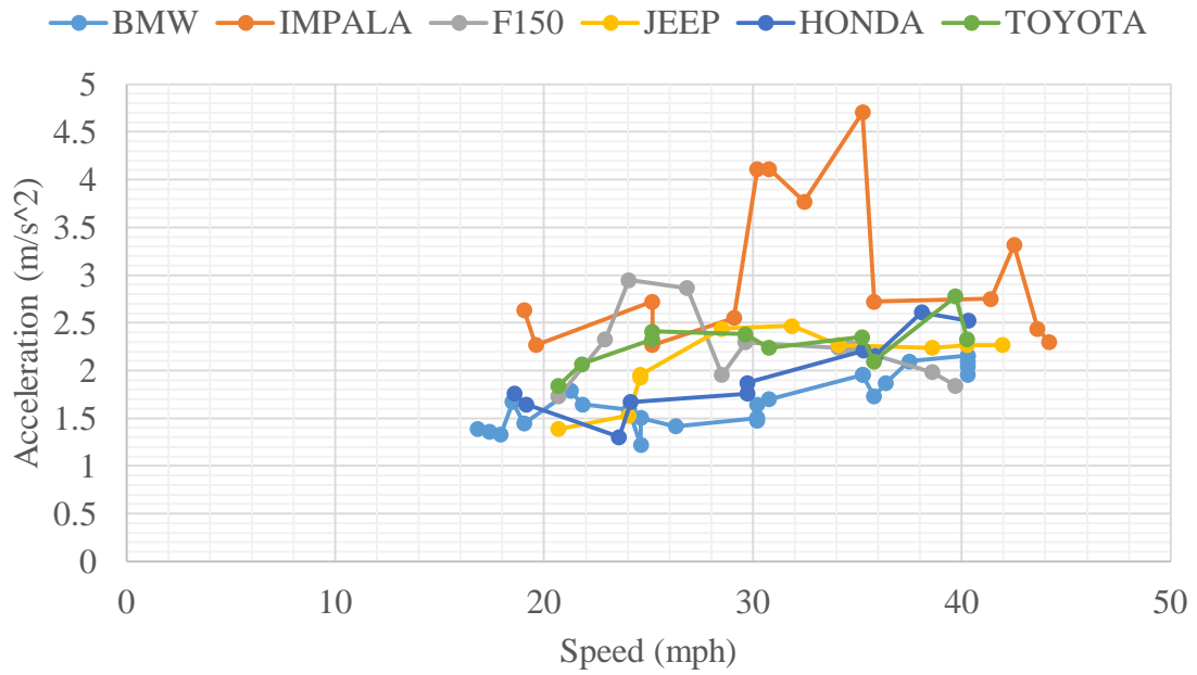
Bryan Station Road Maximum Positive Acceleration West
