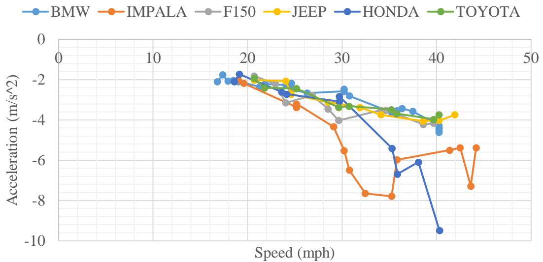
Bryan Station Road Maximum Negative Acceleration West
