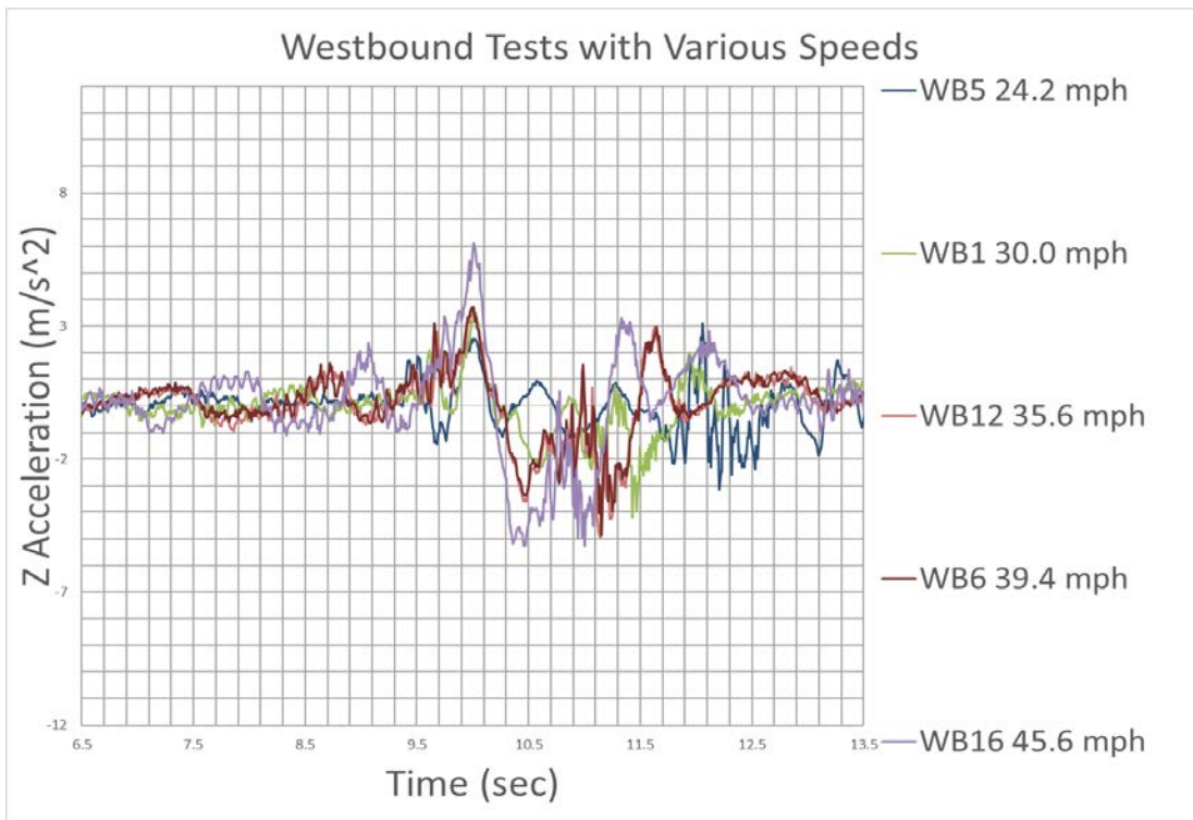
Figure 4.10 Westbound tests with various speeds.
