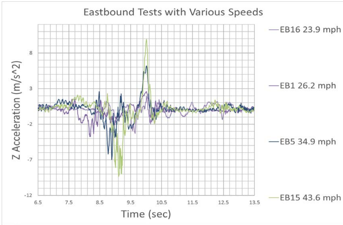
Figure 4.9 Eastbound tests with various speeds.
